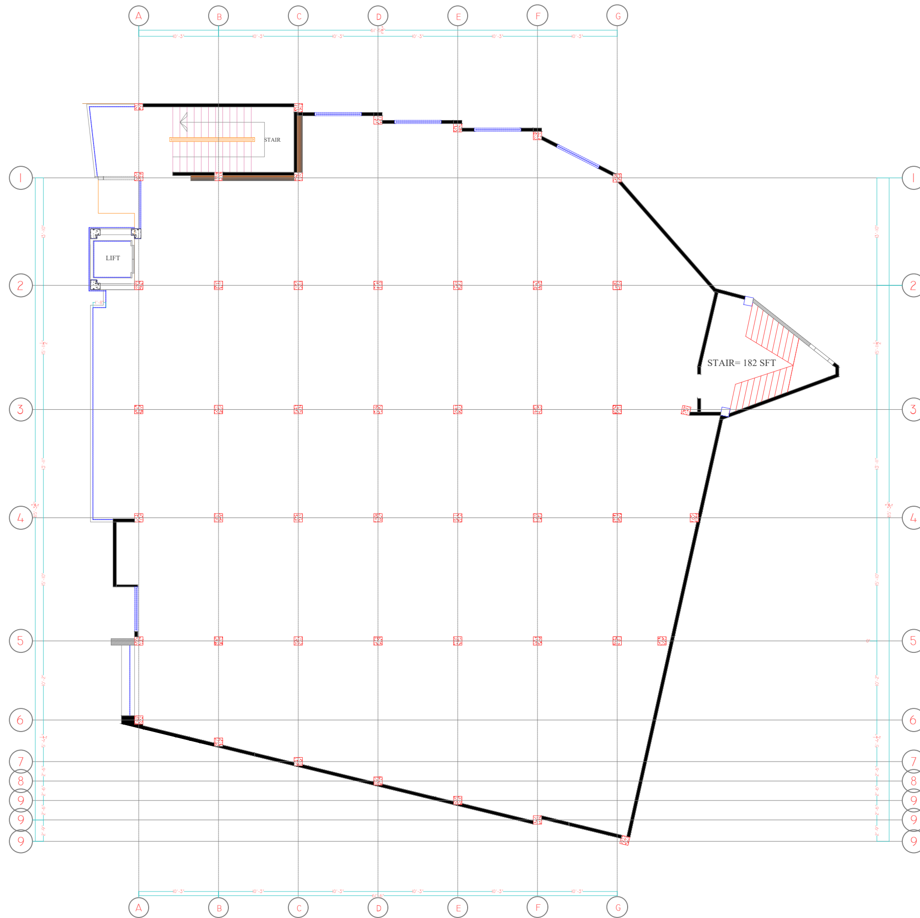
FLOOR LAYOUT
